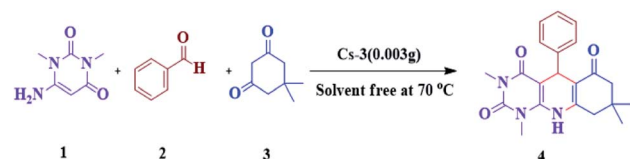
Scheme 1 Model reaction for the synthesis of pyrimido[4,5- b ]quinoxalines 4a .
