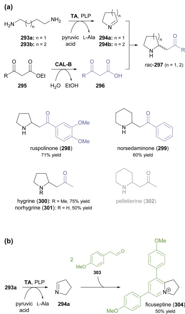
Scheme 38 Use of putrescine transaminase in alkaloid synthesis: (a) biocatalytic formation of cyclic imines 294 from linear diamines 293 and decarboxylative Mannich reaction with in situ generated β-ketoacids 296 affords racemic pyrrolidine and piperidine alkaloids 297 . (b) 1-Pyrroline ( 294a ) formed by transaminase catalysis reacts with two molecules of aldehyde 303 to give the 2,3-dihydroindolizinium alkaloid ficuseptine ( 304 ).
