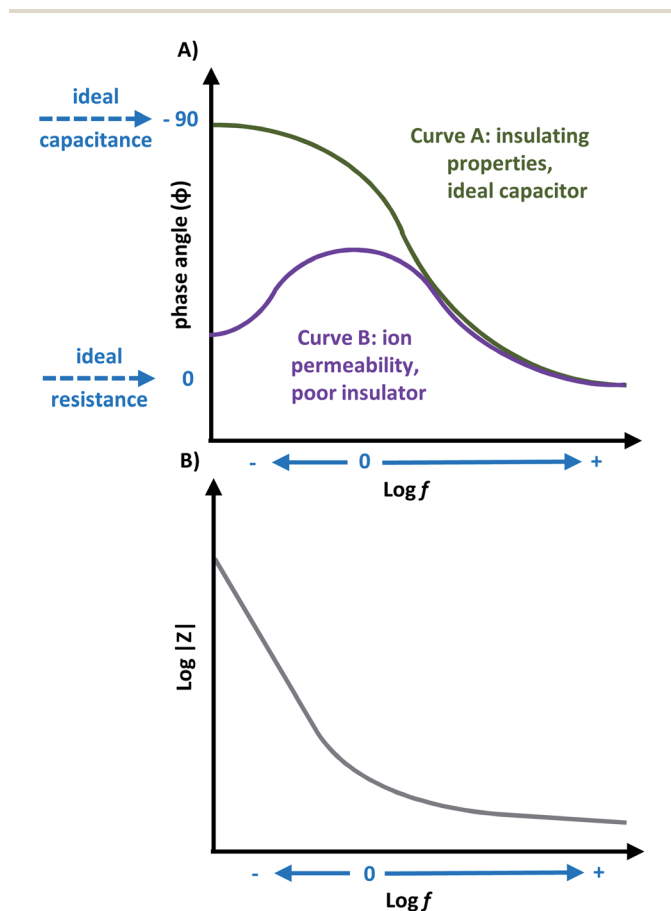
Fig. 9 (A) Sample curve responses for a Bode phase angle plot. (B) Sample Bode magnitude plot.
