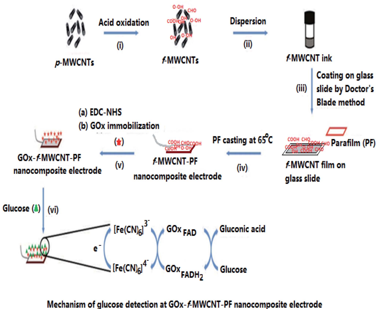
Fig. 1 Schematic of the steps involved in the fabrication of the f-MWCNT–PF nanocomposite-based glucose biosensor.
