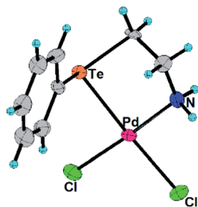
Fig. 1 ORTEP diagram of complex 1 with 50% thermal ellipsoids. Selected bond lengths (Å): Te–Pd: 2.5057(6), Te–C aryl : 2.118(6), Te–C alkyl : 2.149(6), Pd–Cl: 2.3142(16), Pd–N: 2.063(5). Selected bond angles (°): Cl–Pd–Te: 88.82(4), Cl–Pd–Cl: 94.42(6), N–Pd–Te: 88.21(13), N–Pd–Cl: 88.54(14).
