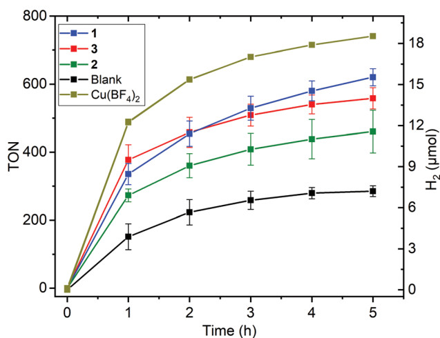
Fig. 5 Hydrogen evolution (TON left, \mu\text{mol} right; see Fig. S12† for this plot in terms of hydrogen volume in mL) vs. time profile for copper complexes 1 [\text{Cu}^{\text{II}}\text{L}^{\text{Et}}]\text{BF}_4 (blue), 2 [\text{Cu}^{\text{II}}\text{L}^{\text{Et-MePy}}]\text{BF}_4 (green), and 3 [\text{Cu}^{\text{II}}\text{L}^{\text{EtPy}_2}]\text{BF}_4 (red), as well as for the blank run with no copper catalyst (black) and the control experiment using the simple \text{Cu}(\text{BF}_4)_2 salt as the copper catalyst (olive), in DMF ( C_{\text{cat}} = 5 \mu\text{M} ) on irradiation with a blue LED ( \lambda = 445 \text{ nm} , 88 \text{ mW cm}^{-2} ) at 20^\circ\text{C} , with 1.0 M TEOA, 0.2 mM [\text{Ru}(\text{bpy})_3](\text{PF}_6)_2 and 0.1 M \text{HBF}_4/0.53 \text{ M H}_2\text{O} . Error bars show the standard deviation from the mean, calculated in Origin from multiple separate runs (Tables 2, S1 and Fig. S14–S17†).
