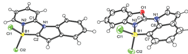
Fig. 2 Solid state structures of left, 4-Cl , and right 17-Cl , ellipsoids at 50% probability. Selected distances (Å) and angles ( ^\circ ) for 4-Cl : B1–N2 = 1.589(2); C2–B1 = 1.587(2); B–C1 = 1.856(1), B1–C12 = 1.848(2); N1–C1 = 1.375(2) N1–C1–N2 = 109.7(1) ; N1–C2–B1 = 107.3(1) ; N2–B1–C2 = 97.7(1) ; C1–N2–B1 = 111.8(1) . For 17-Cl : N2–B1 = 1.561(6); C7–B1 = 1.595(7); B1–C1 = 1.875(6); B1–C12 = 1.861(6); N1–C1 = 1.334(5); N1–C1–N2 124.0(4) ; C1–N2–B1 = 125.2(4) ; C7–B1–N2 = 107.7(4) ; C1–N1–C8 = 118.7(4) .
