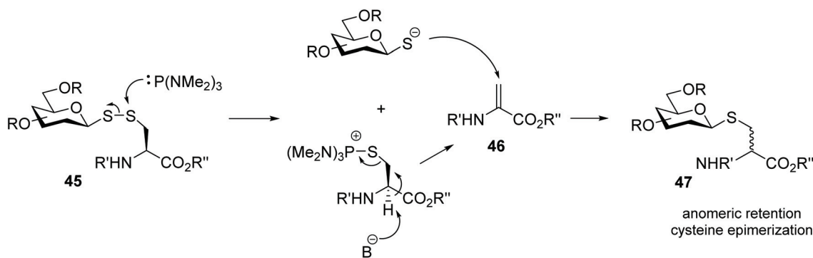
Scheme 15 Proposed S γ -attack followed by elimination-conjugate addition mechanism of desulfurisation of a disulfide-linked glycosyl cysteine.
