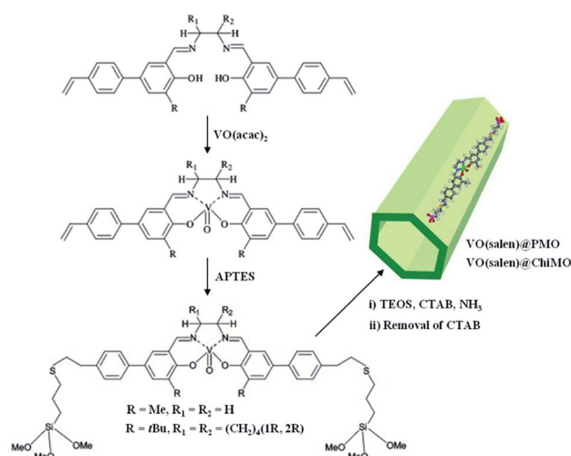
Fig. 6 Preparation of the organosilica precursor and V-incorporated PMOs, \text{VO}(\text{salen})@PMO and \text{VO}(\text{salen})@ChiMO . 78 Reproduced with permission. 78 Copyright 2004, Elsevier.
