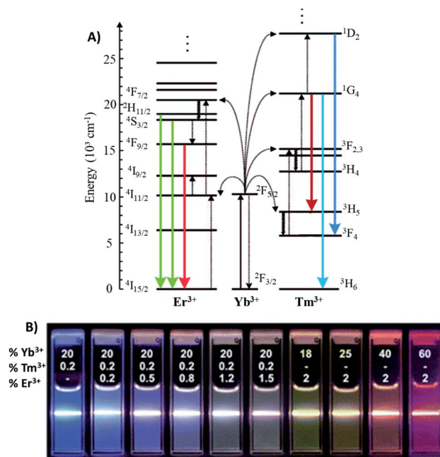
Fig. 1 (A) Energy-level diagram of anti-Stokes processes in UCNPs ( \text{NaYF}_4:\text{Yb,Er/Tm} ). The sensitizer ion \text{Yb}^{3+} absorbs most of the NIR light, and the activator ions \text{Er}^{3+} or \text{Tm}^{3+} emit UV-visible light. Full arrows: radiative transitions, dotted arrows: non-radiative energy transfer, curled arrows: multiphonon relaxation. Modified with permission from ref. 11. Copyright 2004, Wiley-VCH Verlag GmbH & Co. KGaA, Weinheim. (B) Luminescence photographs showing the corresponding colloidal solutions of \text{NaYF}_4 nanoparticles doped with varied concentrations of \text{Yb}^{3+} , \text{Er}^{3+} and \text{Tm}^{3+} , excited at 980 nm, with a 600 mW diode laser. Modified with permission from ref. 13. Copyright 2008, American Chemical Society.
