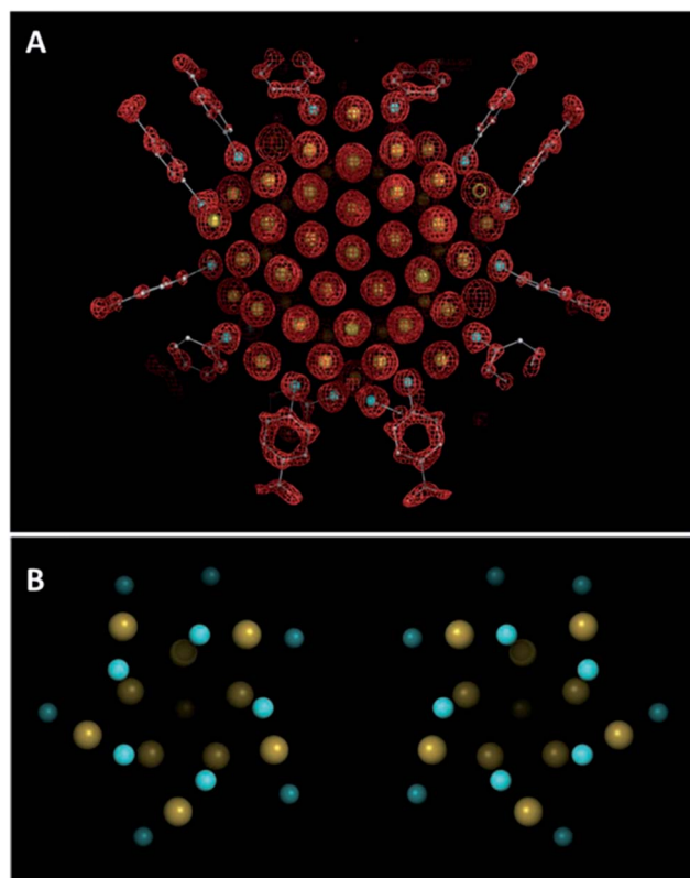
Fig. 2 X-ray crystal structure of the \text{Au}_{102}(\text{p-MBA})_{44} crystal. (A) Electron density map and atomic structure (Au atoms depicted as yellow spheres, and p-MBA shown as framework and with small spheres [S in cyan, C in gray, and O in red]). (B) Top view of the two enantiomeric clusters. Colour scheme as in (A), only the sulfur atoms of p-MBA are shown. Adapted with permission from ref. 48. Copyright 2007 American Association for the Advancement of Science.
