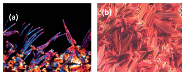
Fig. 6 (a) Microphotograph of the optical texture seen for the ligand LCL-4 at 125 ^\circ\text{C} , wherein the typical textural patterns such as a dark field of view, filaments and focal-conics respectively pertaining to \text{SmA} , TGB and \text{N}^* phases coexist. (b) The focal-conic fan texture of the \text{LmX}^* phase ( 150 ^\circ\text{C} ) for LC-GNP-4.
