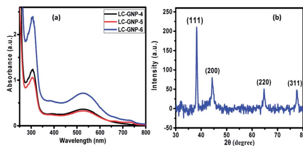
Fig. 4 (a) UV-Vis absorption spectra acquired for DCM solutions of LC-GNPs; notice bands arising due to n-\pi^* ( \sim 300\text{ nm} ) transition and SPR ( \sim 530\text{ nm} ) pertaining into GNPs. (b) Representative XRD pattern of the as-prepared LC-GNP-4.
