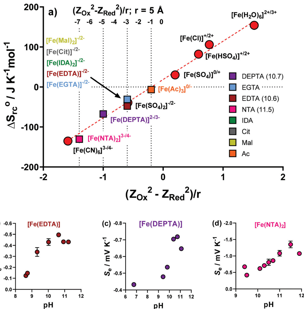
Fig. 7 Showing (a) a plot of \Delta S_{rc}^{\circ} vs. (Z_{\text{Ox}}^2 - Z_{\text{Red}}^2)/r for previously reported aqueous Fe(II)/Fe(III) redox systems (red circles) and all Fe(ligand) solutions investigated here (coloured squares). The dotted lines indicate the (Z_{\text{Ox}}^2 - Z_{\text{Red}}^2) values of 0/-1, -1/-2, -2/-3 and -3/-4 redox couples (using r = 5 \text{ \AA} ). From these the likely ionic charge changes in the redox couples have been put next to the complex, e.g. [\text{Fe}(\text{NTA})_2]^{3-/4-} . The values for Fe(EDTA), Fe(DEPTA) and Fe(NTA) were the pH optimised values (pH values specified in brackets in the legend); (b), (c) and (d) plot the observed trends in S_e vs. pH for these three, respectively, using an applied \Delta T = 20 \text{ K} . pH modification was achieved by the direct addition of solid \text{K}_2\text{CO}_3 to the semi-optimised systems.
