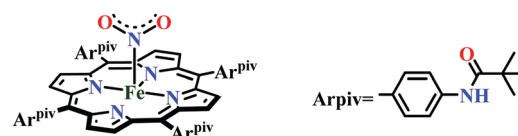
Fig. 15 Molecular structure [(\text{TpivPP})\text{Fe}(\text{NO}_2)]^- .
