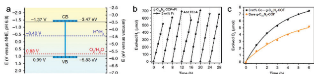
Fig. 24 (a) Bandgap diagram with marked potential for HER and OER. (b) Hydrogen and (c) oxygen production during photocatalytic water splitting based on \text{g-C}_{40}\text{N}_3 -COF. Reproduced with permission. 27 Copyright 2019, Nature Publishing Group.
