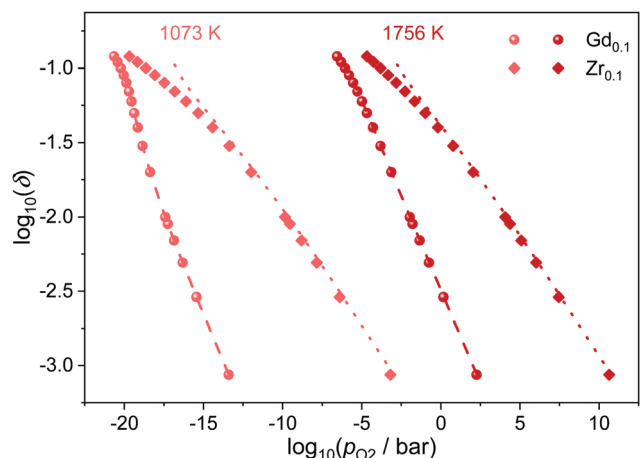
Fig. 6 Relation between oxygen partial pressure and non-stoichiometry in \text{Ce}_{0.9}\text{Gd}_{0.1}\text{O}_{1.9-\delta} and \text{Ce}_{0.9}\text{Zr}_{0.1}\text{O}_{2-\delta} at 1073 K and 1756 K. Symbols represent the results for ordered Gd (spheres) and Zr (diamonds); lines represent the results for the random distribution of Gd (dashed) and Zr (dotted).
