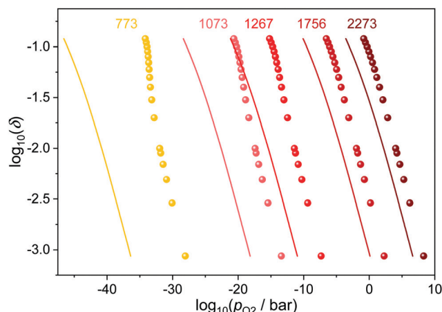
Fig. 5 Relation between oxygen partial pressure and non-stoichiometry in \text{Ce}_{0.9}\text{Gd}_{0.1}\text{O}_{1.9-\delta} for different temperatures. The ideal behavior according to eqn (4) is indicated by the respective lines.
