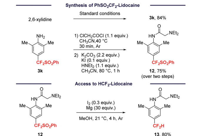
Scheme 7 Synthesis of PhSO 2 CF 2 -Lidocaine and the post-functionalization reaction.
