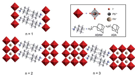
Fig. 1 Schematic representation of adamantyl-based layered hybrid perovskites based on the S_2FA_{n-1}Pb_nI_{3n+1} ( n = 1-3 ; S = ADAM or A, ADA or A') composition. ADAM = (1-adamantyl)methan ammonium; ADA = 1-adamantyl ammonium.
