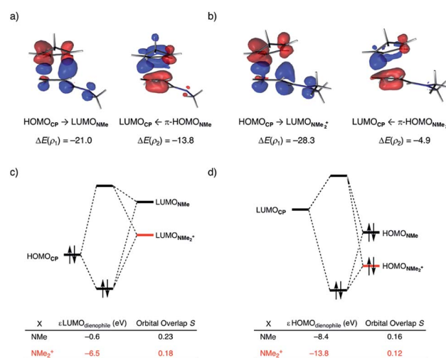
Fig. 7 NOCV deformation densities \Delta\rho (isovalue = 0.0015 \text{ au} ) and associated energies \Delta E(\rho) (in kcal mol -1 ) for the normal electron demand (NED), \text{HOMO}_{\text{CP}}\text{-LUMO}_{\text{dienophile}} , and inverse electron demand (IED), \text{LUMO}_{\text{dienophile}}\text{-HOMO}_{\text{CP}} , where the color flow is red \rightarrow blue, for (a) \text{NMe} , (b) \text{NMe}_2^+ ; the Kohn-Sham molecular orbital analysis for (c) NED, and (d) IED. All data were computed at consistent geometries with a \text{C}_{\text{CP}} \cdots \text{C}_\beta bond length between CP and the dienophile of 2.125 \text{ \AA} at ZORA-M06-2X/TZ2P//M06-2X/def2-TZVP.
