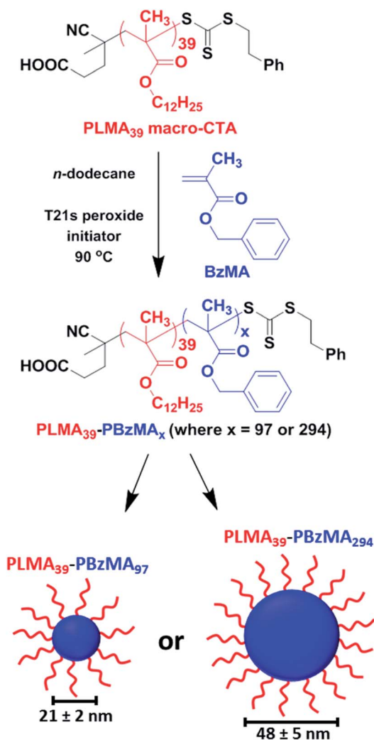
Scheme 1 A \text{PLMA}_{39} precursor block is chain-extended with BzMA monomer in n -dodecane via RAFT-mediated PISA to form sterically-stabilized spherical nanoparticles. SAXS analysis (see Fig. S3, Tables S2 and S3 in the ESI†) indicated that final PBzMA DPs of 97 and 294 produced mean core diameters of 21 \pm 2 nm and 48 \pm 5 nm, respectively.
