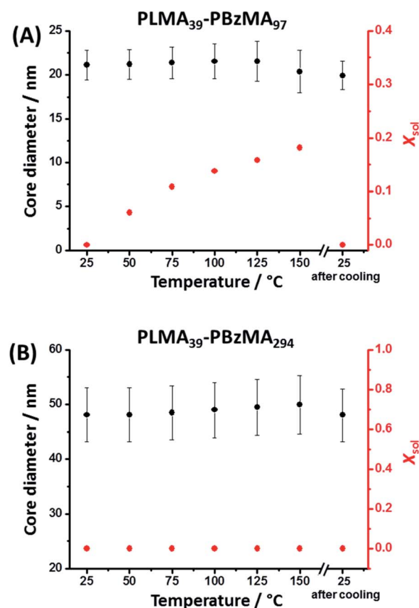
Fig. 1 Mean nanoparticle core diameter and solvent volume fraction ( X_{\text{sol}} ) determined for (A) \text{PLMA}_{39}\text{-PBzMA}_{97} and (B) \text{PLMA}_{39}\text{-PBzMA}_{294} spheres at various temperatures using SAXS analysis (Tables S2 and S3,† respectively). The core diameter remains approximately constant for both types of nanoparticles when heated up to 150 °C. However, progressively higher X_{\text{sol}} values are observed on heating \text{PLMA}_{39}\text{-PBzMA}_{97} spheres. The original X_{\text{sol}} value of approximately zero is obtained for this system on returning to 25 °C. In contrast, \text{PLMA}_{39}\text{-PBzMA}_{294} spheres exhibit no discernible change in X_{\text{sol}} on heating up to 150 °C. [N.B. Error bars correspond to the standard deviation in the mean nanoparticle diameter.]
