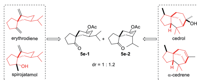
Scheme 2 New synthetic strategy design toward corresponding sesquiterpenes.
