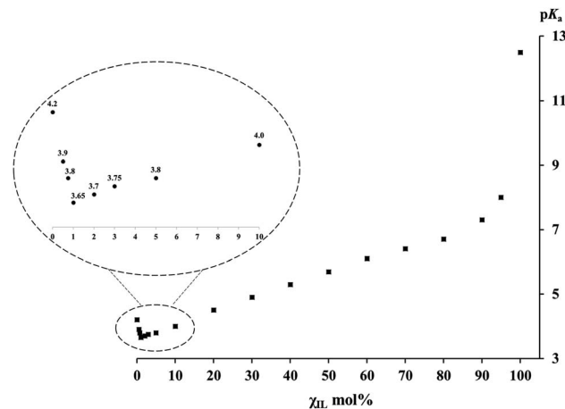
Fig. 1 \text{p}K_{\text{a}} values of \text{PhCH}(\text{CN})_2 versus the molar fractions \chi_{\text{IL}} of [Bmim][NTf 2 ] in [Bmim][NTf 2 ]/DMSO mixtures.
