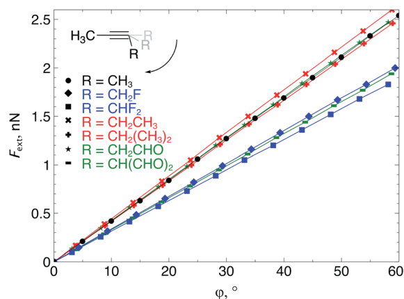
Fig. 4 The required bending force in alkynes increases linearly with the bending angle \varphi , according to eqn (5) but clearly varies upon substitution.
