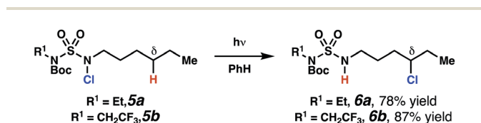
Scheme 2 Chlorine-transfer from “internal” sulfamide nitrogen occurs through a 1,5-HAT process to provide \delta -chlorinated alkanes.
