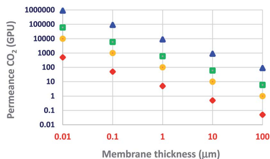
Fig. 3 \text{CO}_2 permeance as a function of membrane thickness: triangle, PIM-1; square, 6FDA-DAM; circle, Pebax® 1657; rhombus, polysulfone. 29,41–43
