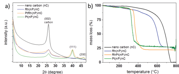
Fig. 1 (a) XRD patterns (CuK \alpha ) of the three composite materials Rh(nP)/nC (blue trace), PtRh(nP)/nC (orange trace), and Pt(nP)/nC (green trace) in comparison to the carbon starting material (nC, black trace). (b) Thermogravimetric analysis (TGA) of the three composite materials and the starting carbon material between 50–800 °C under synthetic air (80% N 2 , 20% O 2 ) with a heating ramp of 10 °C min -1 .
