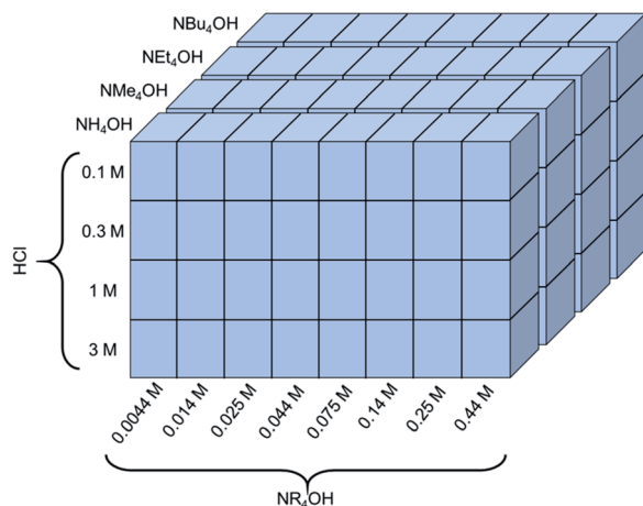
Fig. 2 A schematic of the experimental space used to investigate the dependence of proton concentration, \text{NR}_4^+\text{OH} concentration, and \text{NR}_4^+ ionic radius on the exfoliation yield of LCO.
