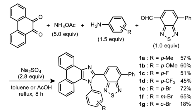
Scheme 1 Synthesis of phenanthroimidazolybenzothiadiazoles 1a–g .
