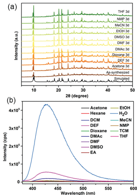
Fig. 3 (a) Solvent stability of \text{CaNH}_2\text{PTA} (ROD-95) monitored using PXRD patterns after immersion for 3 days; (b) selective sensing of water monitored using the emission spectra of \text{CaNH}_2\text{PTA} in supernatants of various solvents in 1 min.
