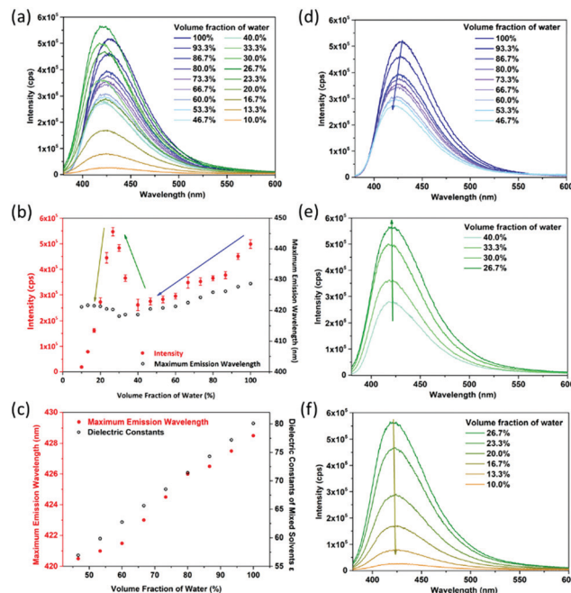
Fig. 4 Luminescence sensing of the water content in DMF through self-disintegration of \text{CaNH}_2\text{PTA} (ROD-95): (a) emission spectra with different water contents, (b) luminescence intensity and maximum emission wavelength as a function of water volume fraction, (c) the relationship between maximum emission wavelength and dielectric constants, and (d–f) emission spectra of the three segments.
