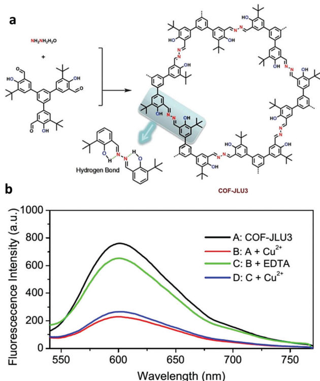
Fig. 20 (a) Synthesis of COF-JLU3 depicting the intramolecular hydrogen bonding. (b) Fluorescence spectra of COF-JLU3 demonstrating its effective reversible quenching by Cu 2+ ions. Adapted from Chem. Commun. , 2016, 52, 6613, with permission from the Royal Society of Chemistry.
