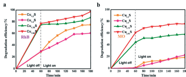
Fig. 5 Photocatalytic activities of \text{Cu}_{2-x}\text{S} for RhB (a) and MO (b) photodegradation under UV irradiation.
