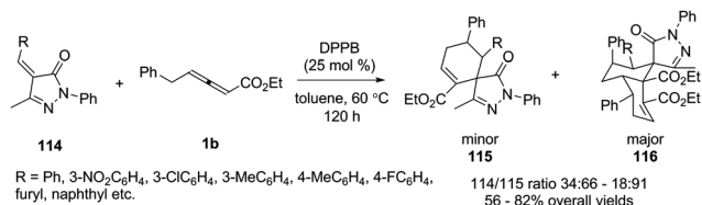
Scheme 36 Bisphosphine-catalysed sequential annulation of an allenate with benzylidenepyrazolones.
