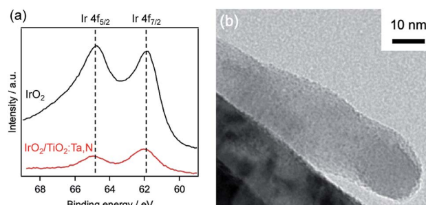
Fig. 10 Characterization of 1.0 wt% \text{IrO}_2 -loaded \text{TiO}_2\text{:Ta,N} . (a) Ir 4f XPS spectrum and (b) TEM image.
