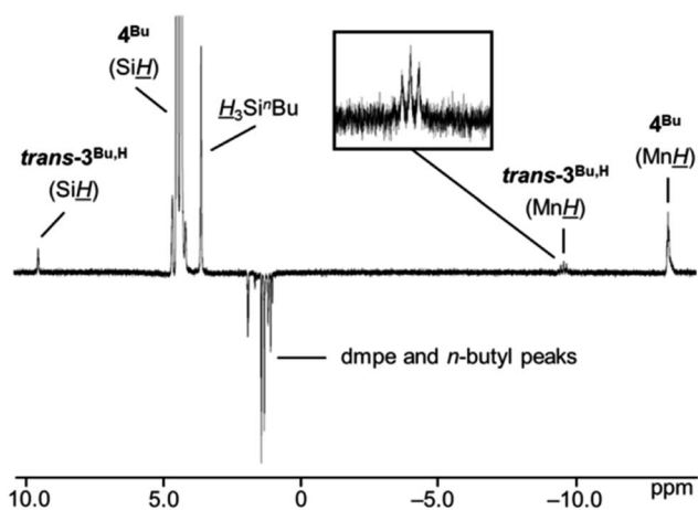
Fig. 6 1D NOESY/EXSY NMR spectrum of a solution of [(dmpe) 2 -MnH(SiH 2 n Bu) 2 ] (4 Bu ) at 335 K with excitation at the SiH signal of 4 Bu , showing chemical exchange between the SiH and MnH environments of [(dmpe) 2 MnH(SiH 2 n Bu) 2 ] (4 Bu ) and trans -[(dmpe) 2 MnH(=SiH n Bu)] ( trans -3 Bu,H ), and the SiH environment of free H 3 Si n Bu. Positive (EXSY) peaks are indicative of chemical exchange and negative (NOESY) peaks are indicative of through-space coupling (500 MHz, C 6 D 6 ).
