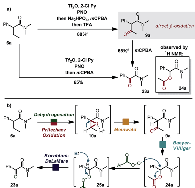
Scheme 6 (a) Alternative pathway towards different ketoamides. See ESI† for detailed reaction conditions. (b) Proposed mechanism.
