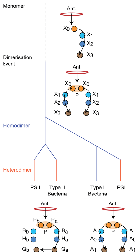
Fig. 2 Evolution of reaction centres (RC). 1 The primordial RC was monomeric, likely comprising three BChls ( X_0 , X_1 , X_2 ) and a quinone ( X_3 ). An antenna (Ant.) would transfer an exciton to X_0 , which would also serve as the charge donor. The charge would transfer through X_1 and X_2 before arriving at X_3 . The monomeric RC dimerised, producing a homodimer with two identical copies of the monomer, connected at the special pair (P). Excitons from the antenna could delocalise over P before charge separation, with charge transfer occurring along either branch. The homodimer subsequently diverged into type I and type II RCs, some of which experienced gene duplication events that led to heterodimerism. In modern type I RCs, each branch consists of three (B)Chls (P, A, and A_0 ) and a quinone ( A_1 ). In heterodimeric PSI, charge transfer occurs exclusively down one branch, while in homodimeric systems (such as heliobacteria) charge can move down either branch with equal probability. In modern type II RCs, each branch consists of two (B)Chls (P and B), a phaeophytin (H) and a quinone (Q). Charge travels down one branch before being transferred to the inactive-branch quinone.
