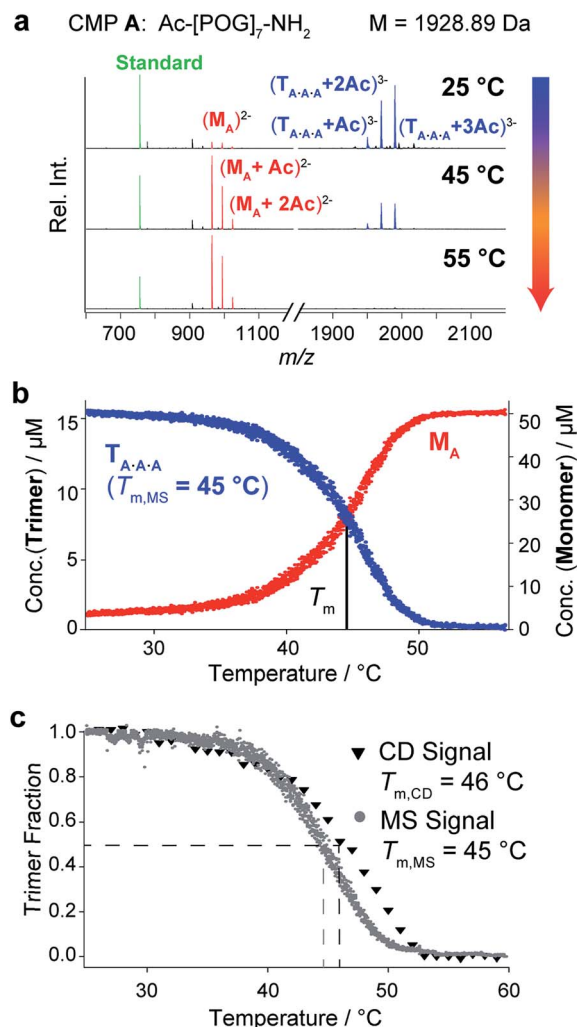
Fig. 2 CD spectroscopic and native MS analyses of CMP A (50 \mu M in 10 mM aq. NH_4Ac at pH 7). (a) MS spectra of CMP A at different temperatures. The observed m/z signals correspond to the triply charged trimers (blue), the doubly charged monomers (red), and the internal standard (10 \mu M bradykinin 1–7, green). (b) Thermal denaturation profile of CMP A obtained by monitoring the monomer and trimer m/z signals as a function of temperature (heating rate: 1 °C min^{-1} ). (c) Overlay of the normalized thermal denaturation curves of CMP A obtained by using CD spectroscopy (triangles) and MS (dots) as monitoring tools (heating rate: 1 °C min^{-1} ).
