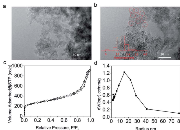
Fig. 1 TEM (a) and HRTEM (b) images, N 2 sorption isotherms (c) and pore size distribution (d) of the Pd/C catalyst used in this work.
