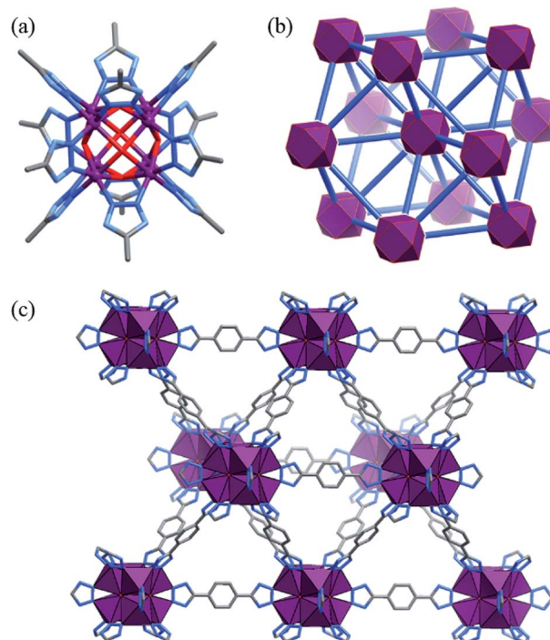
Fig. 1 (a) The \text{Co}_8(\mu_4\text{-OH})_6(\text{Rtrz})_{12} cluster (hydrogen atoms are omitted for clarity), (b) the network topology (octanuclear clusters and bistriazolate ligands are simplified as violet polyhedra and blue sticks, respectively), and (c) 3D coordination framework ( \text{CoN}_3\text{O}_3 units are shown as violet polyhedra) of \text{Co}_4\text{-bdt} .
