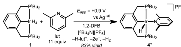
Scheme 2 Electrosynthesis of cationic iridium hydride 4 + .
