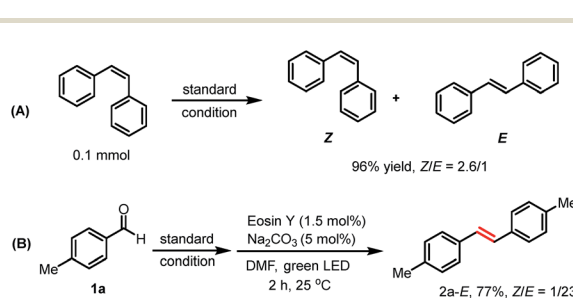
Scheme 4 Isomerization studies.
