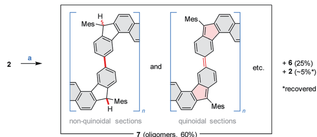
Scheme 4 Thermally induced oligomerization of 2 . Reagents and conditions: (a) argon, pressure tube, 240 °C, 14 h.
