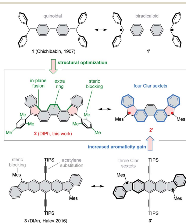
Scheme 1 5,10-Dimesityldiindeno[1,2- a :2',1'- i ]phenanthrene ( 2 ) and its structural relationship to Chichibabin's hydrocarbon ( 1 ) and Haley's diindenoanthracene ( 3 ). Mes = mesityl, TIPS = tri(isopropyl)silyl.
