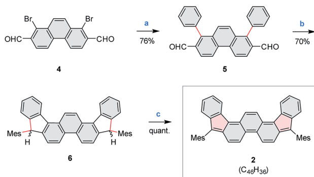
Scheme 2 Synthesis of 5,10-dimesityldiindeno[1,2- a :2',1'- i ]phenanthrene (2). Reagents and conditions: (a) \text{PhB}(\text{OH})_2 , \text{Pd}(\text{PPh}_3)_4 , \text{Na}_2\text{CO}_3 (aq), dioxane, reflux, overnight. (b) (1) \text{MesMgBr} , THF, rt, overnight. (2) \text{BF}_3 \cdot \text{Et}_2\text{O} , DCM, rt, 10 min. (c) 2.5 equiv. DDQ, toluene, rt, overnight.
