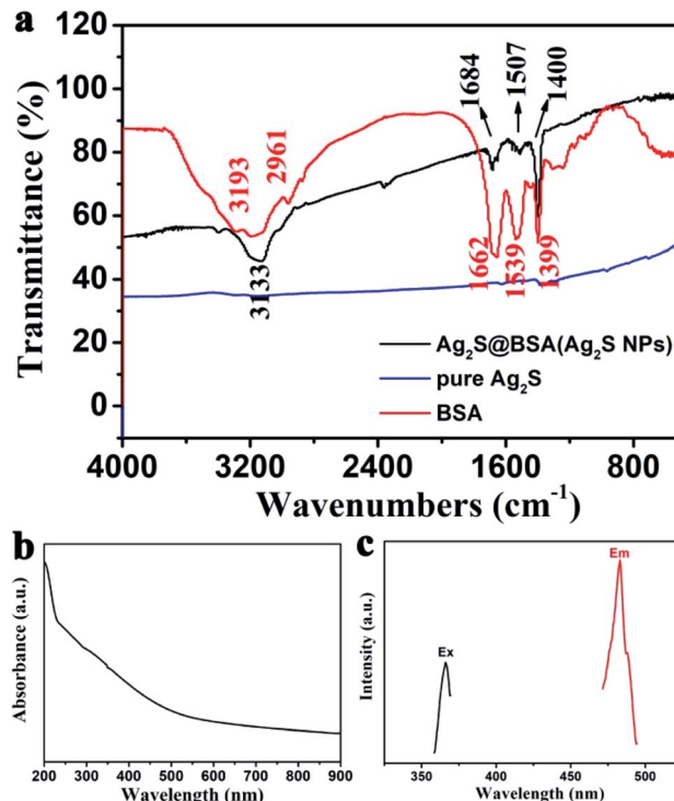
Fig. 2 Optical adsorption and photodynamic properties of \text{Ag}_2\text{S} NPs. (a) FT-IR spectra of \text{Ag}_2\text{S}@BSA ( \text{Ag}_2\text{S} NPs), BSA and pure \text{Ag}_2\text{S} . (b) UV-vis spectrum of \text{Ag}_2\text{S} NPs ( 3.5 \mu\text{g ml}^{-1} ) in aqueous solutions. (c) Fluorescence spectrum of \text{Ag}_2\text{S} NPs ( 3.5 \mu\text{g ml}^{-1} ) in aqueous solution.
