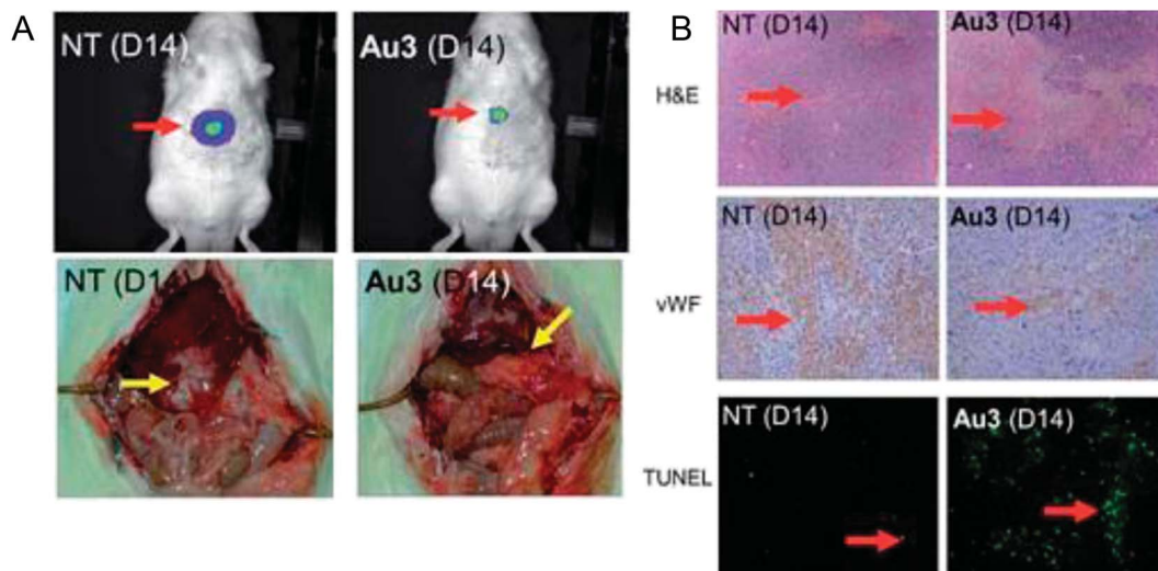
Fig. 28 (A) The sizes of tumor nodules of the vehicle-control (NT, left) or [Au 2 (C N C) 2 (μ-dppp)](CF 3 SO 3 ) 2 -treated (0.5 mg kg -1 ) rat examined by Xenogen Imaging System (upper) and dissection (lower). (B) H&E, vWF, and TUNEL staining of the tumor tissue of vehicle control (NT) and [Au 2 (C N C) 2 (μ-dppp)](CF 3 SO 3 ) 2 -treated (0.5 mg kg -1 ) rats. This figure is reproduced from ref. 150 with permission from the Royal Society of Chemistry (Great Britain).
