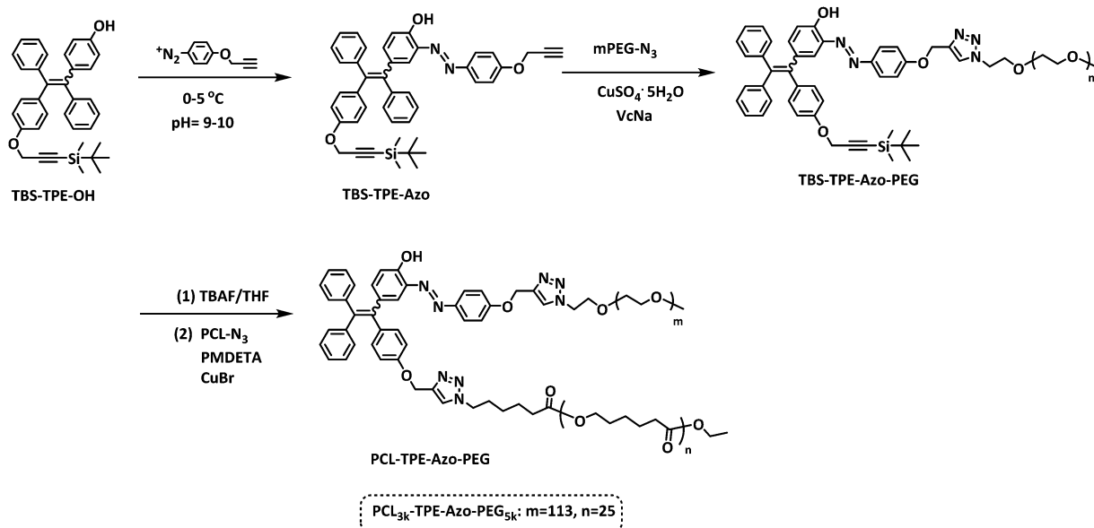
Scheme 1 Synthetic routes of the block copolymer PCL n -TPE-Azo-PEG m .
