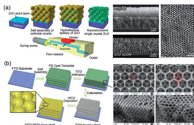
Fig. 3 (a) Flow-reactor-assisted hydrothermal fabrication process and morphologies of 3DOM ZnO. Reproduced with permission. 52 Copyright 2017, American Chemical Society. (b) Fabrication process and morphologies of core-shell 3DOM TiO 2 and TiO 2 -WO 3 . Modified with permission. 53 Copyright 2018, Royal Society of Chemistry.
