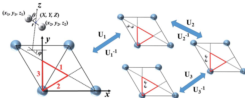
Fig. 1 Cartesian ( x_1, y_1, z_1, x_2, y_2, z_2 ) and internal ( X, Y, Z, r, \theta, \varphi ) coordinates to describe \text{H}_2 interacting with a rigid Ag(111) surface represented by a unit cell, with the symmetry unique triangle marked in red (left panel). Transformation matrices ( U_1, U_2, U_3 ) and their inverses that move a molecular configuration outside the triangle into it and back to the original position, corresponding to the three reflection lines (1, 2, 3) that enclose the triangle.
