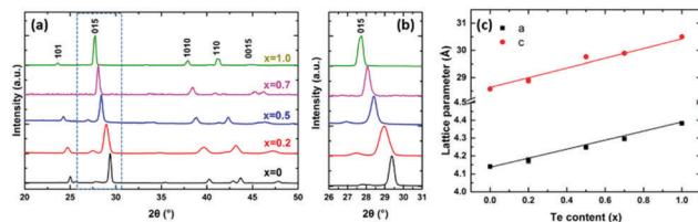
Fig. 4 (a) XRD patterns of as-deposited Bi 2 (Se 1-x Te x ) 3 films with x ranging from 0 to 1; (b) expanded XRD patterns showing the systematic shift of the 015 peak; (c) refined lattice parameters (see Table S1, ESI†) as a function of the Te content for different as-deposited Bi 2 (Se 1-x Te x ) 3 films.
