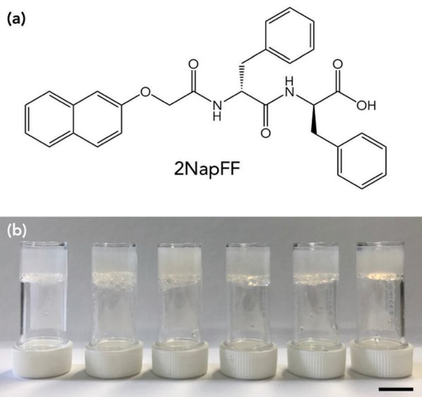
Fig. 1 (a) Chemical structure of gelator 2NapFF. (b) Photographs of 2NapFF at (left to right) 10 mg mL -1 , 5 mg mL -1 , 2.5 mg mL -1 , 20 : 80 glycerol : water (5 mg mL -1 ), 40 : 60 glycerol : water (5 mg mL -1 ) and 60 : 40 glycerol : water (5 mg mL -1 ). Scale bar is 1 cm.
