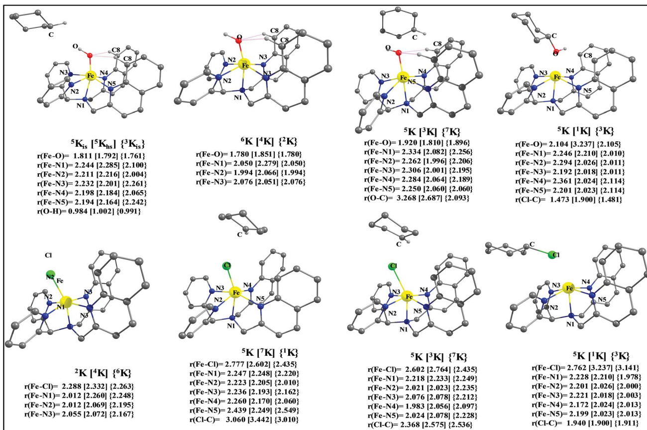
Fig. 14 B3LYP-D2-optimized structures with selected structural parameters: (a) ^{5.5,3}int1 , (b) ^{2.4,6}int2 , (c) ^{3.5,7}ts2 , (d) ^{1,3,5}P + P_{OH} , (e) 2,4,6int3 , (f) ^{3.5,7}int4 , (g) ^{3.5,7}ts3 , and (h) ^{1,3,5}P + P_{Cl} .
